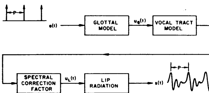
FIGURE 1. Block diagram of a cascade speech synthesizer. (From Markel and Gray. 6 Reprinted by permission.)
