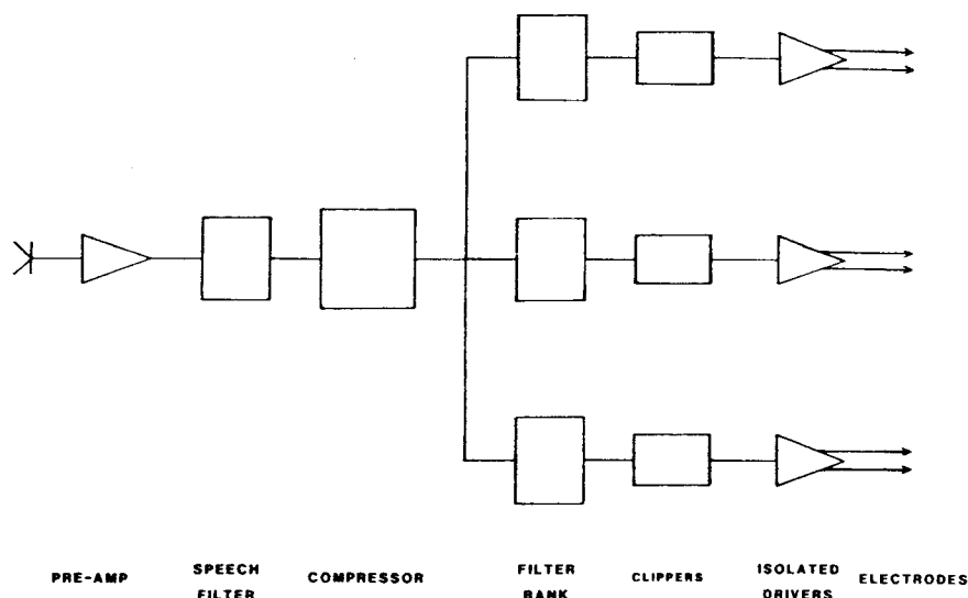
FIGURE 7. Block diagram of CB's three-channel speech-processor. TABLE 7 contains a list of the processor's specifications.
