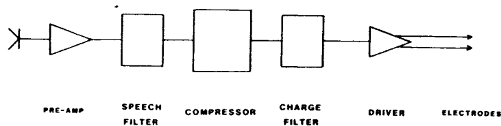
FIGURE 6. Block diagram of CB's single-channel speech-processor. TABLE 6 contains a list of the processor's specifications.
